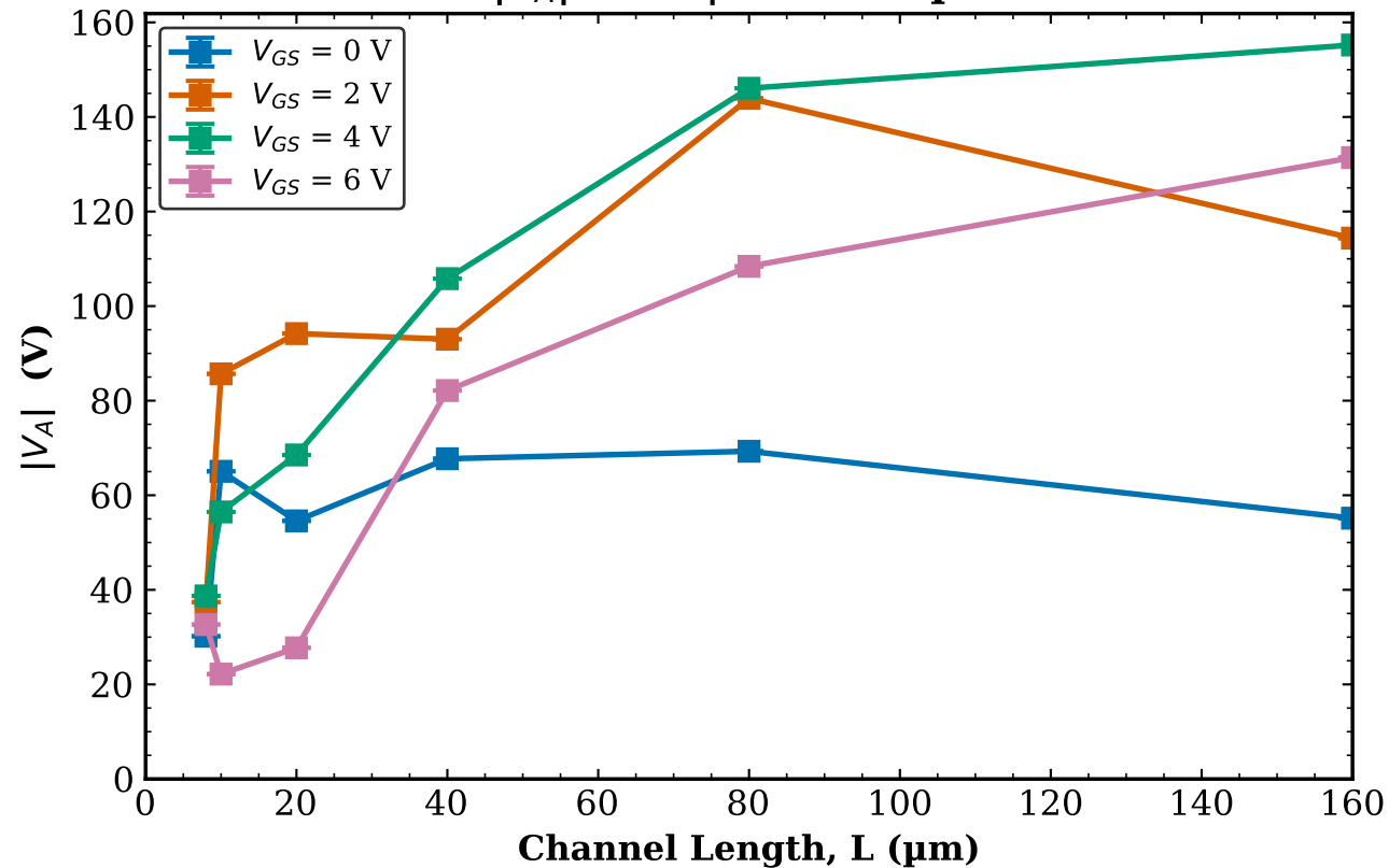
TFT1 Transistor 1 |V_A| vs L | W = 10\text{ }\mu\text{m}
